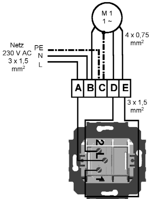
i-Switch
